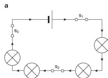
▲ Figure 7.13a Adding an extra bulb in series will result in the bulbs shining less brightly.
