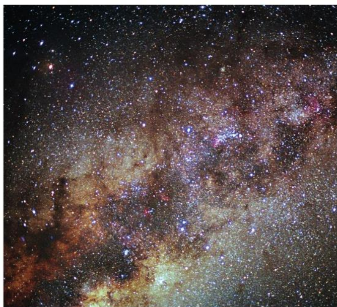
▲ Figure 27.2 Our galaxy, the Milky Way
