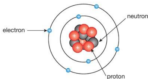
▲ Figure 22.1 A simple model with protons and neutrons in the nucleus of the atom and electrons in orbits around the outside
