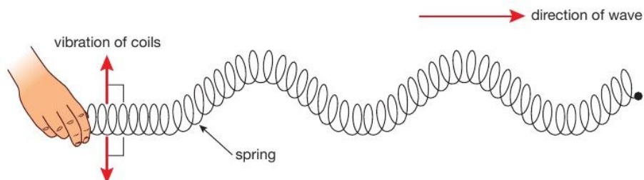
▲ Figure 10.4 A transverse wave vibrates at right angles to the direction in which the wave is moving.
