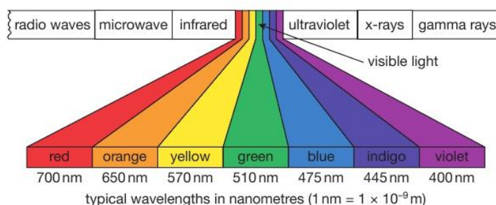
▲ Figure 11.2 The complete electromagnetic spectrum
