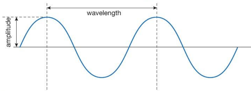
▲ Figure 10.6 A wave has amplitude and wavelength.
