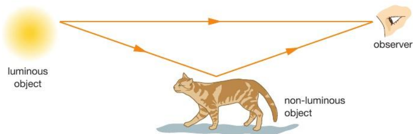
▲ Figure 12.3 Luminous objects, such as the Sun, give out light. Non-luminous objects only reflect light.
