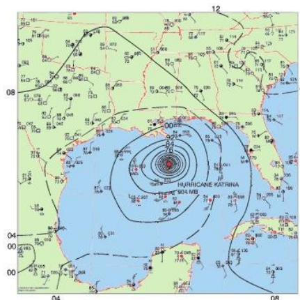
▲ Figure 18.12 Weather maps show isobars (lines of equal air pressure). The centre of hurricane Katrina is a very low pressure region surrounded by isobars that are very close together. The result of the pressure difference is very strong winds.
