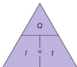
▲ Figure 7.5 You can use the triangle method for rearranging equations like this.
