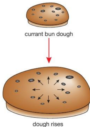
▲ Figure 28.6 As the bun expands the currants get further apart. Similarly as the Universe expands the galaxies get further apart.
