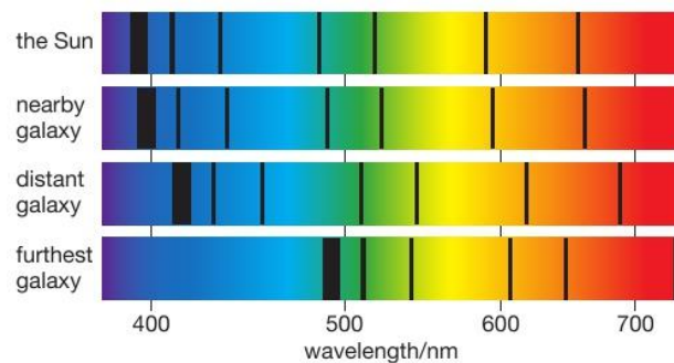
▲ Figure 28.4 Light spectra for four different objects
