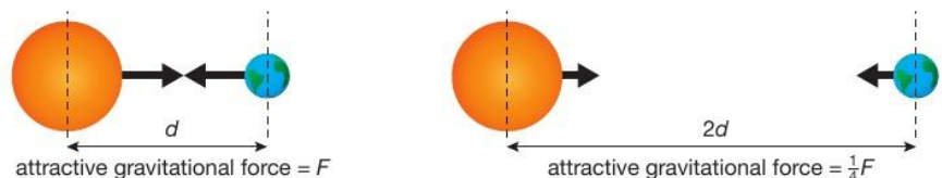
▲ Figure 26.4 Gravitational forces obey an inverse square law – that is, if the distance between the masses is doubled, the forces between them are quartered ; if the distance between them is trebled , the forces become one ninth of what they were.
