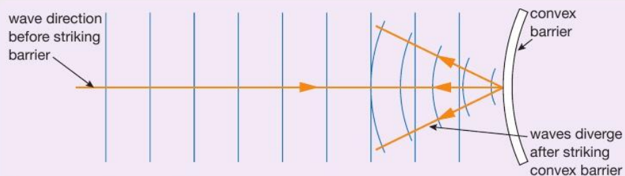
▲ Figure 10.17 Waves striking a convex barrier are reflected backwards and spread out.
