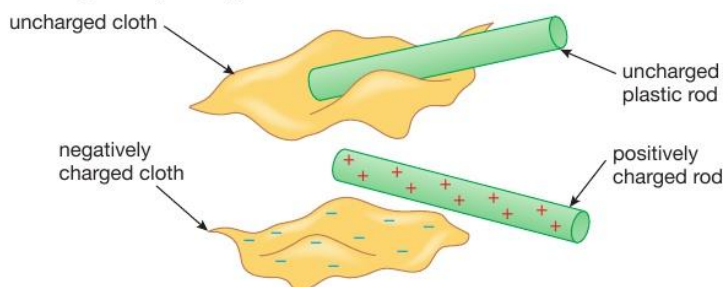
▲ Figure 9.4 Rubbing an uncharged rod with an uncharged piece of cloth can result in them both becoming charged.
