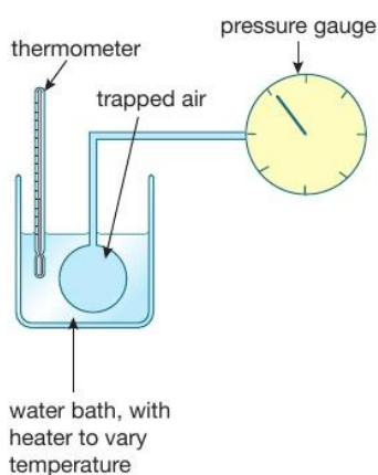
▲ Figure 19.10 Simple apparatus to measure the pressure of a fixed volume of gas at a range of temperatures
