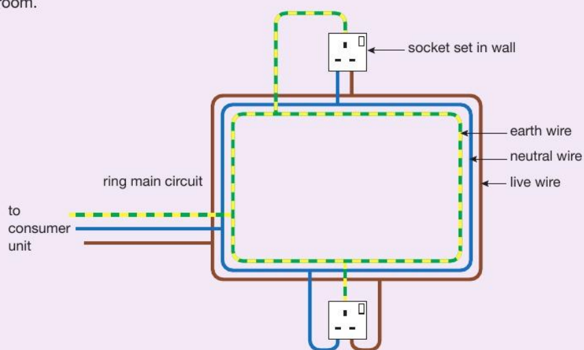
▲ Figure 6.3 Ring main circuits help to cut down on the amount of wiring needed in a house.
