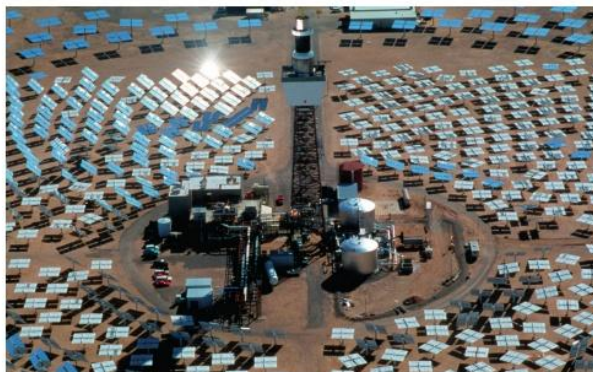
▲ Figure 17.16 A large number of mirrors focus heat from the Sun on a boiler in the tower at the centre. The steam produced drives a turbine to generate electricity.
