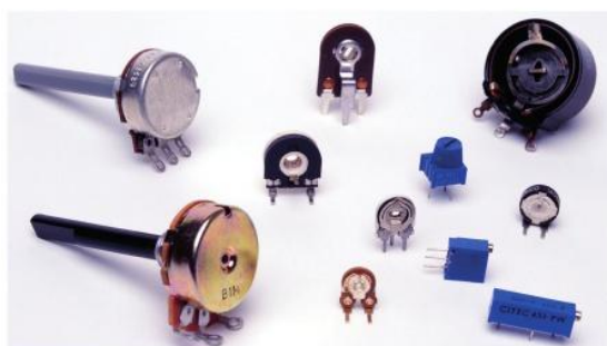
▲ Figure 8.11 Variable resistors and their symbol
