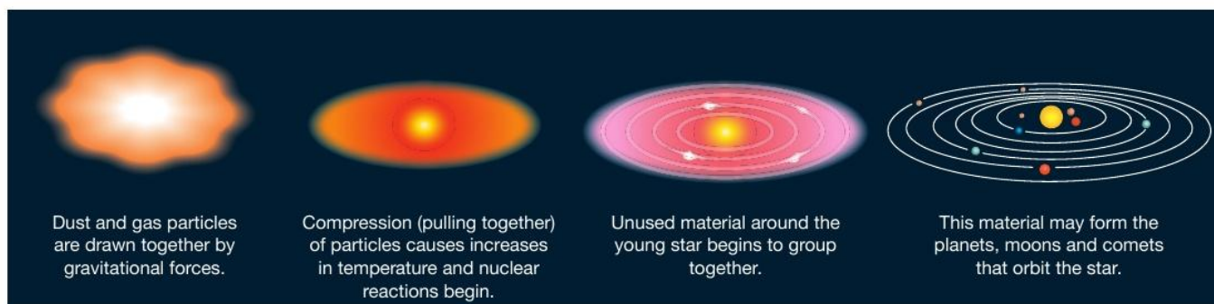
▲ Figure 27.6 Birth of a solar system
