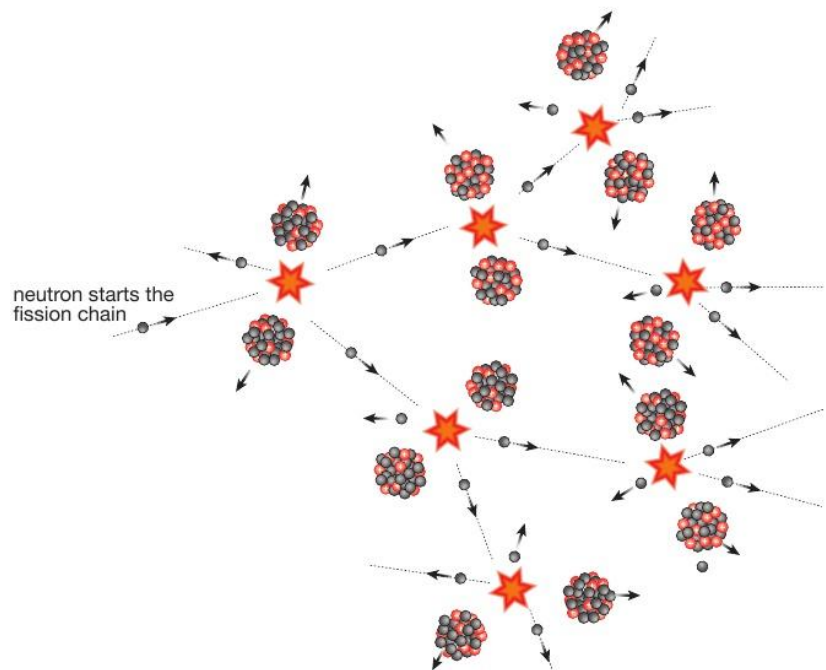
▲ Figure 25.2 A chain reaction in uranium-235
