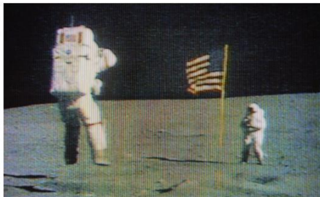
▲ Figure 3.13 An astronaut jumping on the Moon enjoying the effect of low gravity
