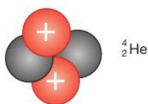
▲ Figure 22.7 An alpha particle ( \alpha particle)
