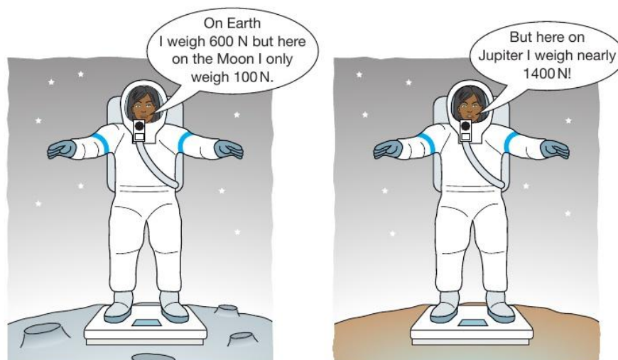
▲ Figure 26.10 The difference in one person's weight on the Moon and on Jupiter
