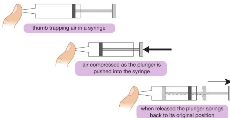
▲ Figure 19.7 Air is squashy!
