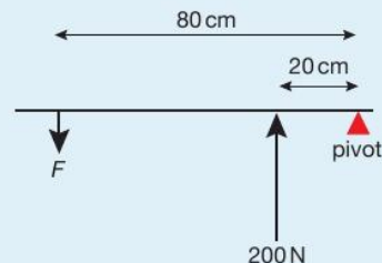
▲ Figure 5.5 A labelled sketch of the problem
