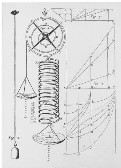
▲ Figure 2.12 Robert Hooke (1635–1703) was a contemporary of Sir Isaac Newton. This is a drawing of the apparatus Hooke used in his experimental work on the extension of a spring.
