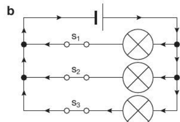
▲ Figure 7.12b A typical parallel circuit. Opening any one of these switches will turn off just the bulb in that part of the circuit.
