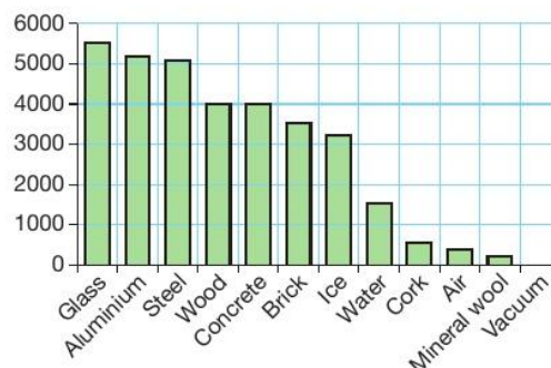
► Figure 13.15 Graph of speeds of sounds (in m/s) for different materials
