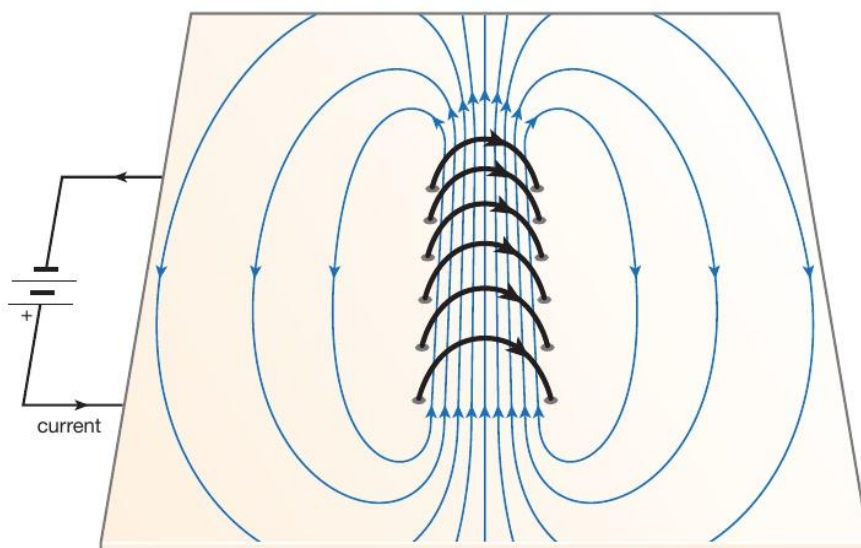
▲ Figure 20.12 The field around a solenoid looks like this.
