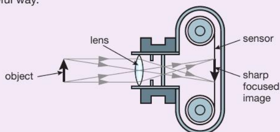
▲ Figure 10.20 In this camera, light waves are refracted by a glass lens to create a sharp image on the sensor or film. Refraction occurs because light travels more slowly in glass than in air.
