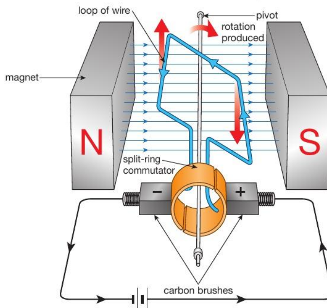
▲ Figure 21.7 A simple electric motor
