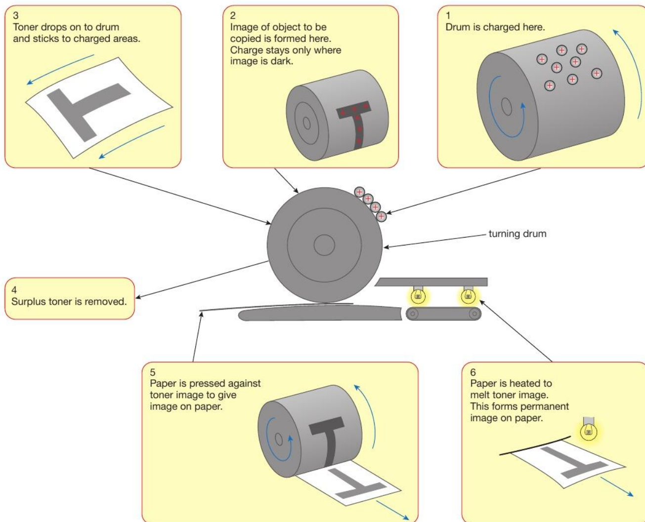
▲ Figure 9.14 Static electricity is used in photocopiers.
