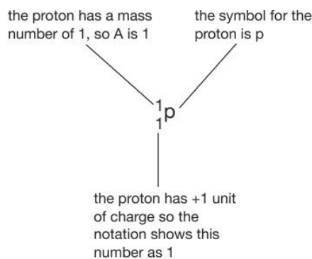
▲ Figure 24.8 The proton
