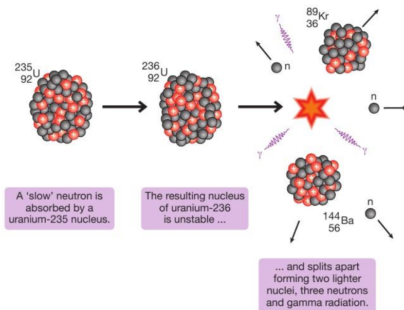
▲ Figure 25.1 One example of fission of uranium-235
