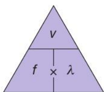
▲ Figure 13.10 The equation triangle for speed, frequency and wavelength.
