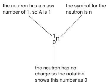
▲ Figure 24.7 The neutron
