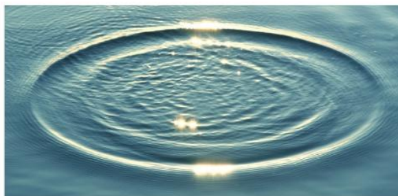
▲ Figure 10.2 Waves are produced if we drop a stone into a pond. The circular wavefronts spread out from the point of impact, carrying energy in all directions, but the water in the pond does not move from the centre to the edges.
