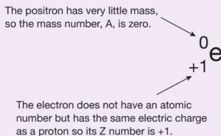
▲ Figure 22.11 A beta plus particle
