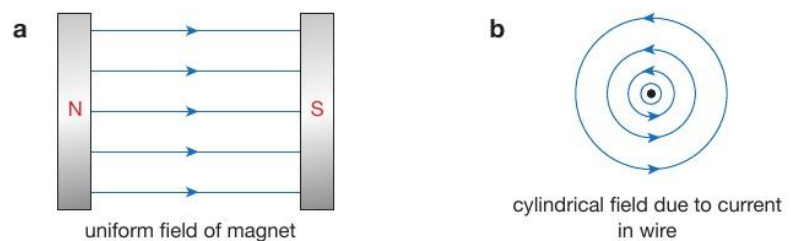
▲ Figure 21.3 a Magnet's uniform magnetic field b Magnetic field around a current carrying wire
