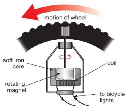
▲ Figure 21.12 A dynamo is a simple generator.
