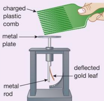
▲ Figure 9.9 A modern gold leaf electroscope
