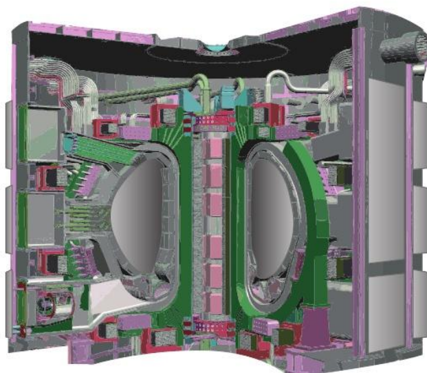
▲ Figure 17.18 Cross-section of a prototype fusion reactor
