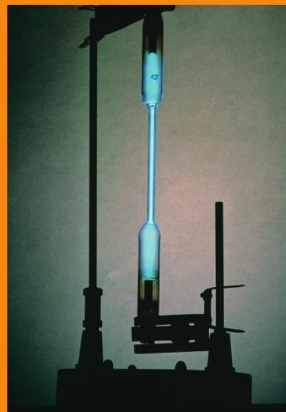
▲ Figure 7.1 The gas in this tube glows when there is a current.
