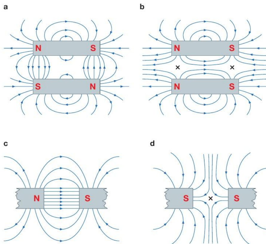
▲ Figure 20.6 Magnetic fields around pairs of magnets
