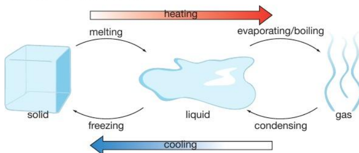
▲ Figure 19.2 Changes of state
