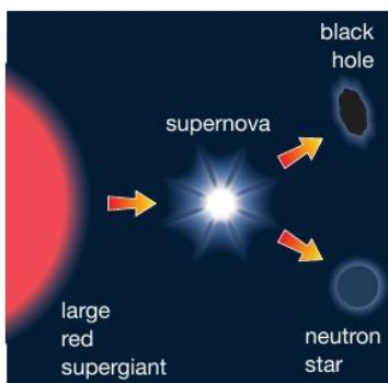
▲ Figure 27.8 The final stages for stars with masses much greater than our Sun
