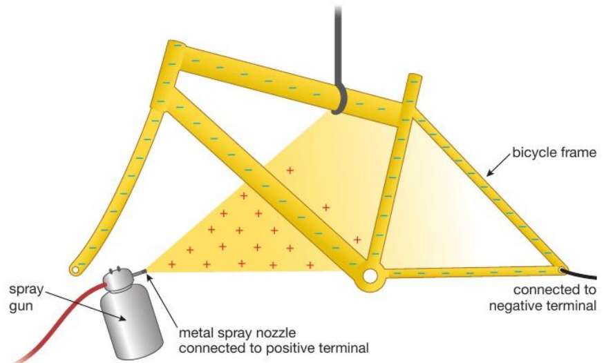
▲ Figure 9.11 The positive paint is attracted to all parts of the negatively charged object.
