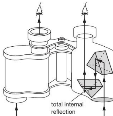
▲ Figure 12.18 Total internal reflection inside binoculars
