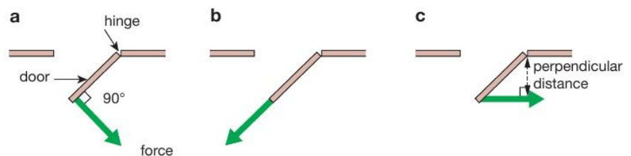
▲ Figure 5.3 For a force to have its biggest effect it should be at 90^\circ to the lever.
