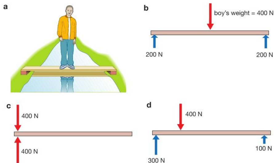
▲ Figure 5.13 The forces at the ends of a beam depend on where the load is applied.
