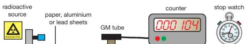
▲ Figure 22.8 Measuring the penetrating power of different types of radiation
