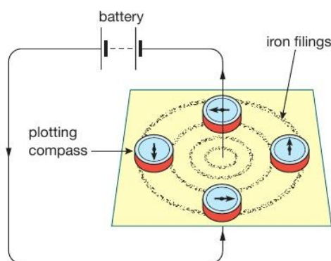
▲ Figure 20.9 A current-carrying wire has a magnetic field around it.
