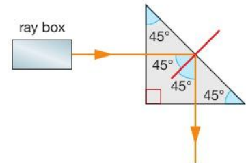
▲ Figure 12.13 Turning through 90^\circ using total internal reflection
