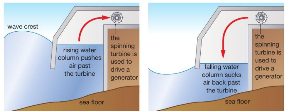
▲ Figure 17.11 An oscillating water column system for using wave energy
