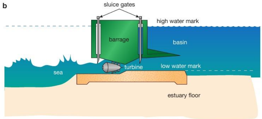
▲ Figure 17.9 a Tidal power station at La Rance, Brittany. b Tidal power also involves harnessing (using) the energy in moving water.
