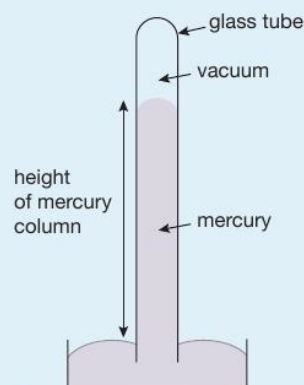
▲ Figure 18.11 A simple mercury barometer
