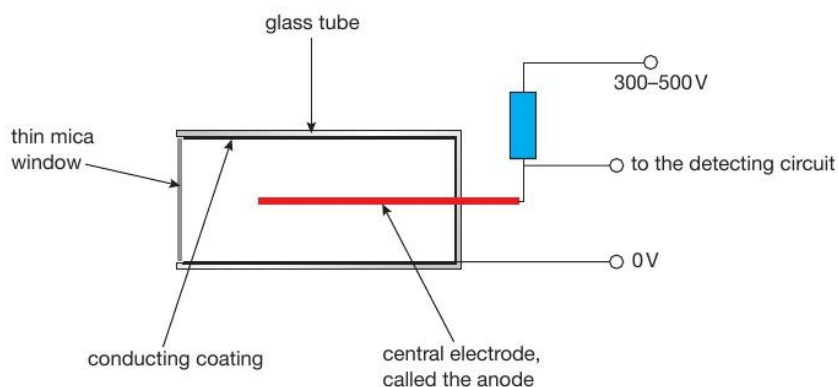
▲ Figure 23.2 A Geiger-Müller tube is used to measure the level of radiation.
