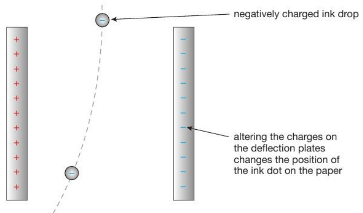
Figure 9.13 The charged ink drops are deflected into the correct position on the paper.
