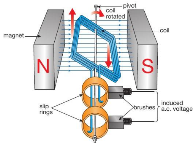
▲ Figure 21.17 The alternator produces alternating current.
