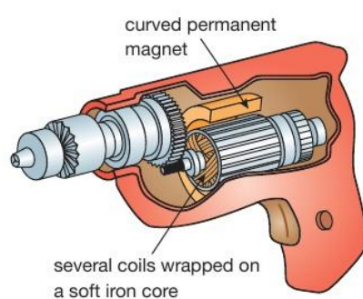
▲ Figure 21.8 A real electric motor
