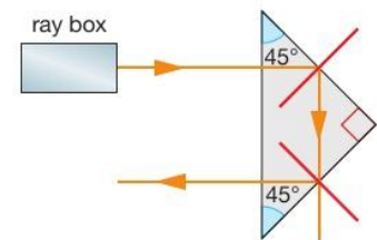
▲ Figure 12.14 Turning through 180^\circ using total internal reflection
