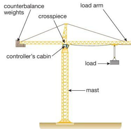
Figure 5.6 The clockwise and anticlockwise moments on the crane must be balanced.
