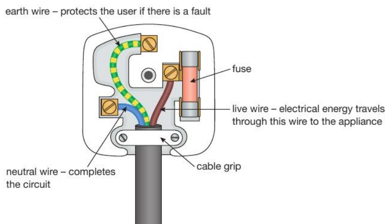
▲ Figure 6.5 A labelled plug
