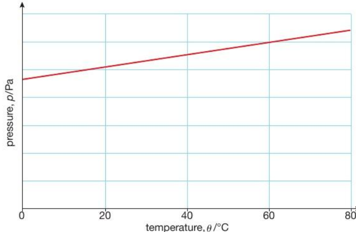
▲ Figure 19.11 Graph to show how the pressure of a fixed volume of gas varies with temperature
