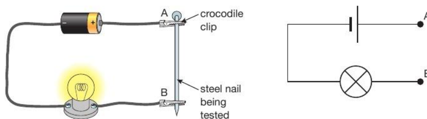
▲ Figure 9.3 Testing circuit
