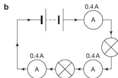
▲ Figure 7.15b The addition of a second cell doubles the voltage applied to the circuit so the current will also double.
